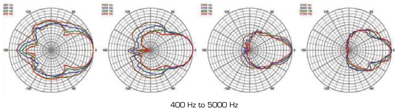
FIGURE 10 - SMS9120 Vertical 1/3 Octave Polar Charts
