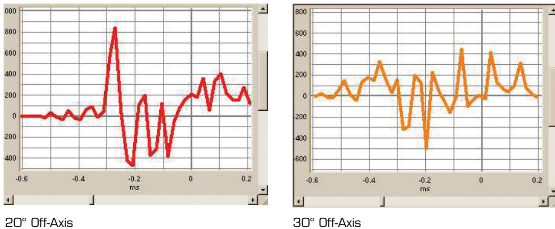
FIGURE 9: SMS9120 Impulses Responses, Vertical Plane
