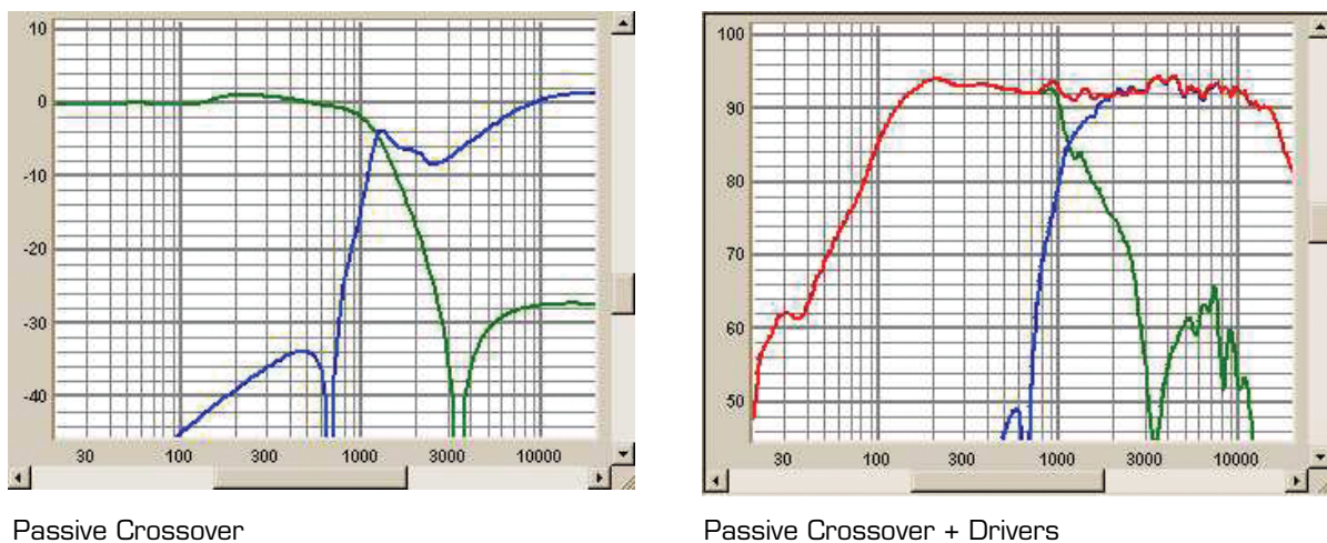
FIGURE 7: SMS9440 Crossover Responses
