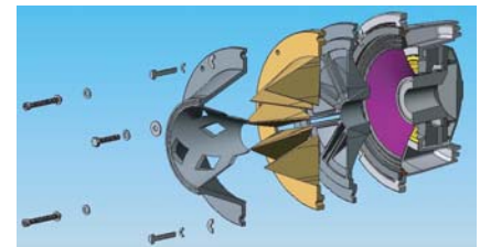
Fig 4 - AX Coaxial Driver
