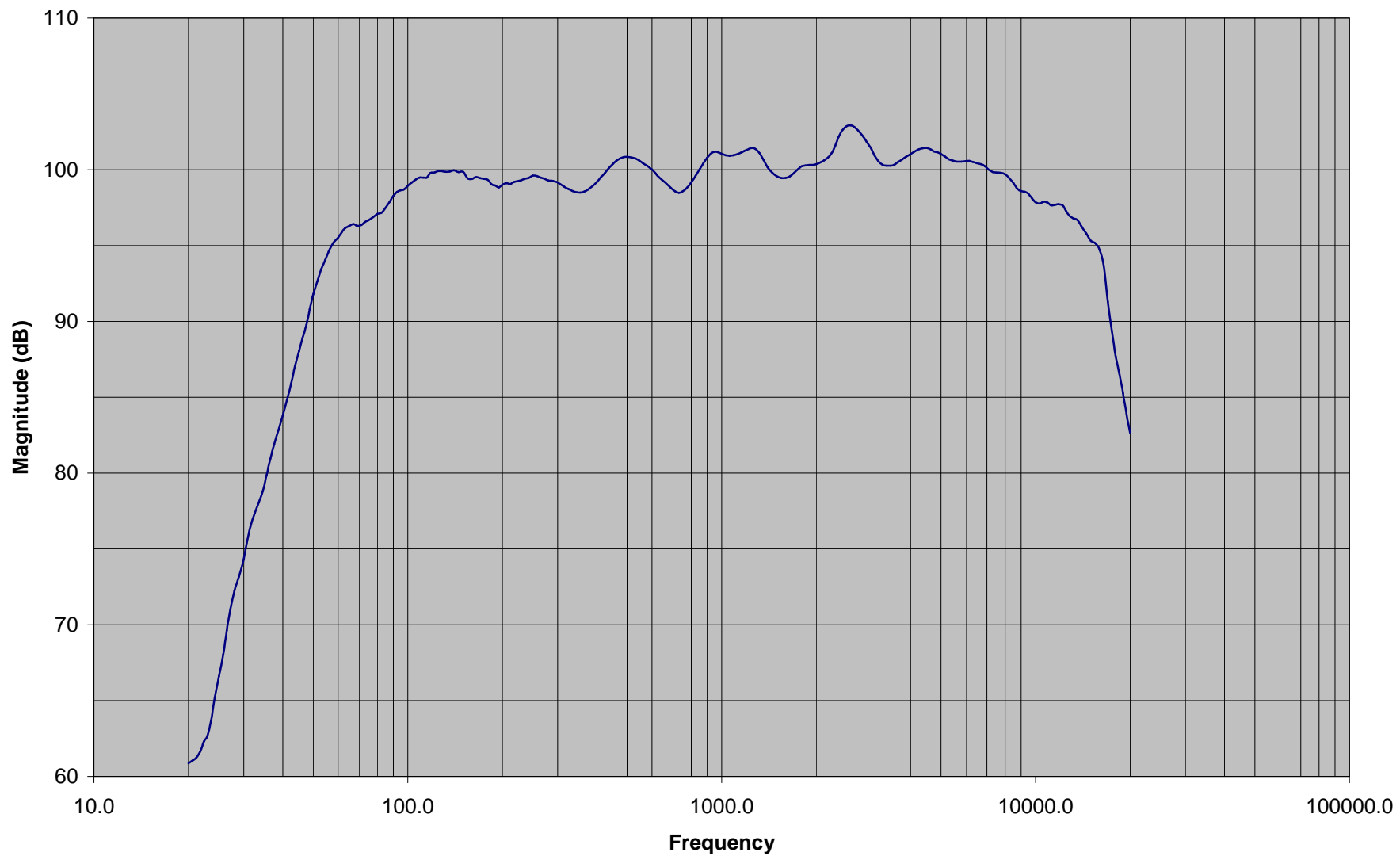
Axial Response (dB SPL/2.83V/1m)
