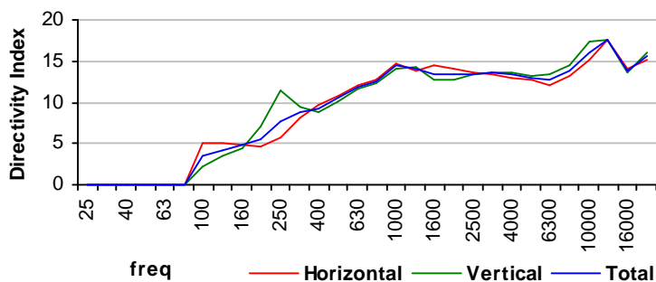
Directivity
