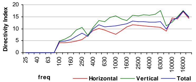
Directivity
