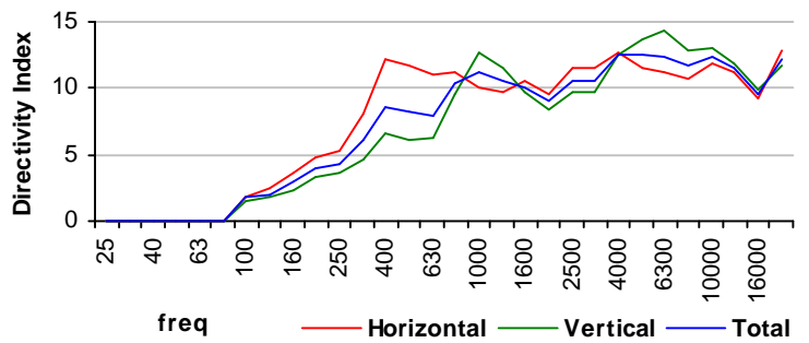
Directivity
